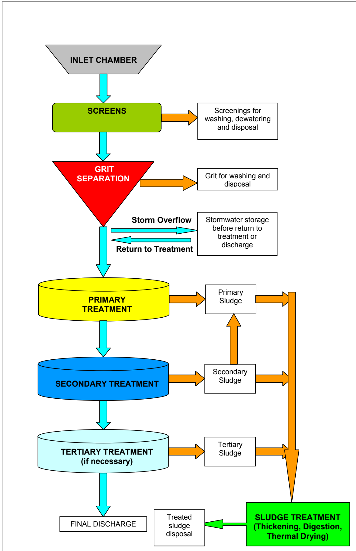
FIGURE 2 – WWTW PROCESS FLOW SHEET
